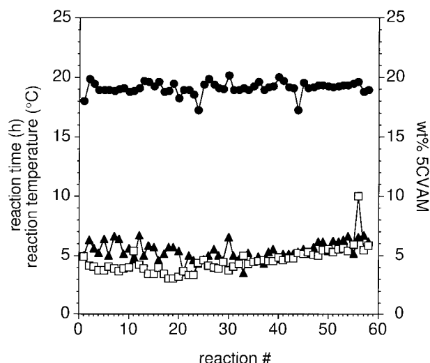
Figure 5. Reaction time ( \square ), average reaction temperature ( \blacktriangle ), and weight % 5CVAM ( \bullet ) for 58 consecutive batch reactions with catalyst recycle to produce a total of 13.6 metric tons of 5CVAM. Reactions were run in two-phase reaction mixtures containing ADN and 5.8% (final weight catalyst/weight reaction mixture) B23/alginate beads in 23 mM sodium butyrate/5 mM calcium chloride (pH 7) at 5°C.
