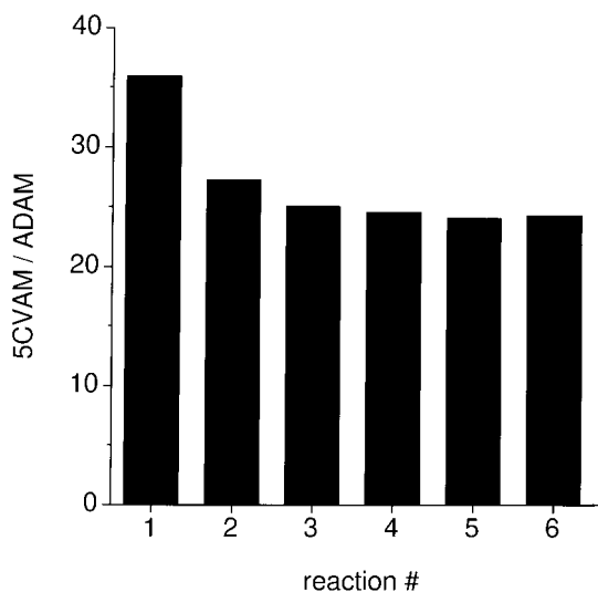
Figure 3. Ratio of 5CVAM/ADAM produced in consecutive batch reactions with recycle of B23/alginate beads. Reactions were run to produce 1.5 M 5CVAM in two-phase reaction mixtures containing ADN and 7.5% (w/w) B23/alginate beads in 23 mM sodium butyrate/5 mM calcium chloride (pH 7.0) at 5°C.
