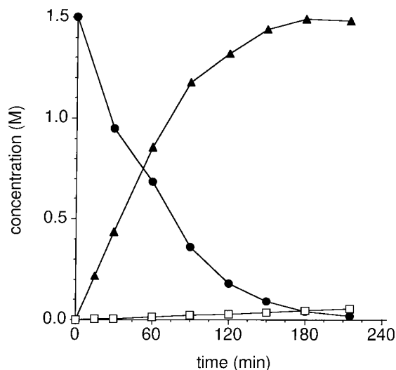
Figure 4. Time course for the production of 1.5 M 5CVAM in a two-phase reaction mixture containing ADN and 7.5% (w/w) B23/alginate beads in 23 mM sodium butyrate/5 mM calcium chloride (pH 7.0) at 5°C: ADN (●), 5CVAM (▲), ADAM (□).
